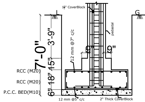
FOOTING F1(SECTION A-A)
