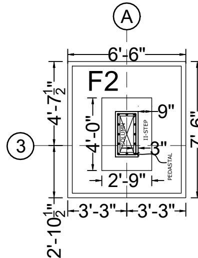
FOOTING F2(PLAN)
