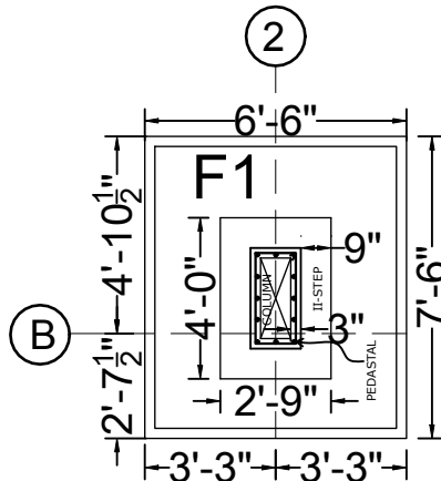
FOOTING F1(PLAN)
