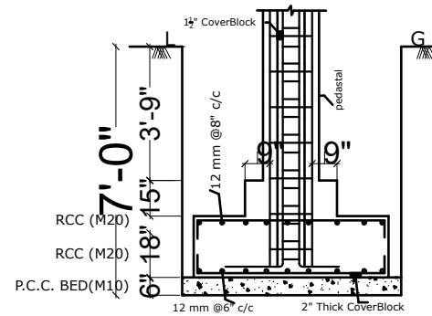
FOOTING F2(SECTION B-B)
