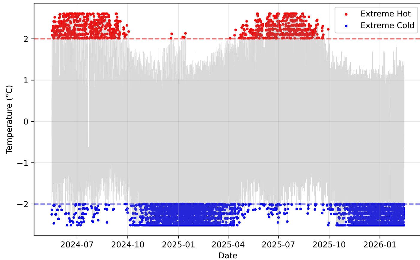
Extreme Weather Events Over Time
