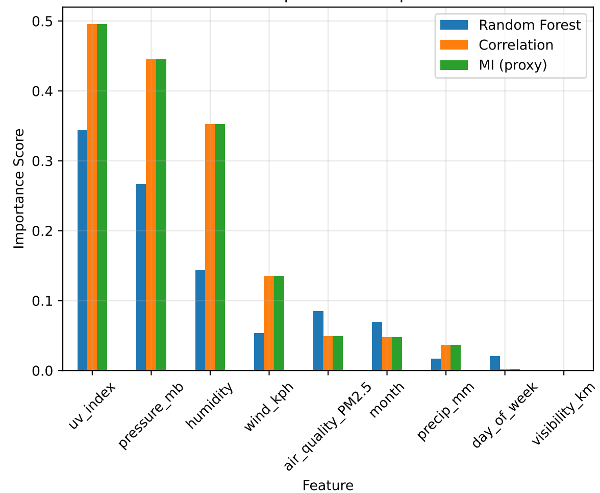
Feature Importance Comparison
