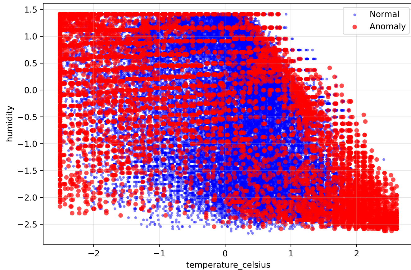
Isolation Forest Anomalies
