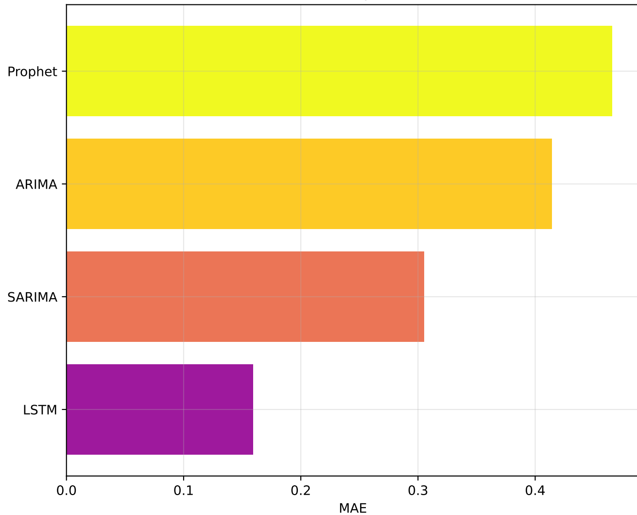
Model Error Comparison (MAE)
