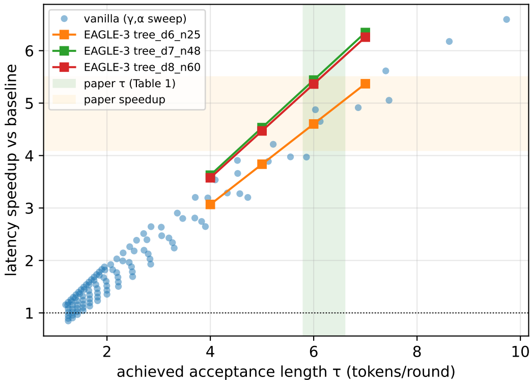
Speedup vs acceptance length (ctx=2048)
