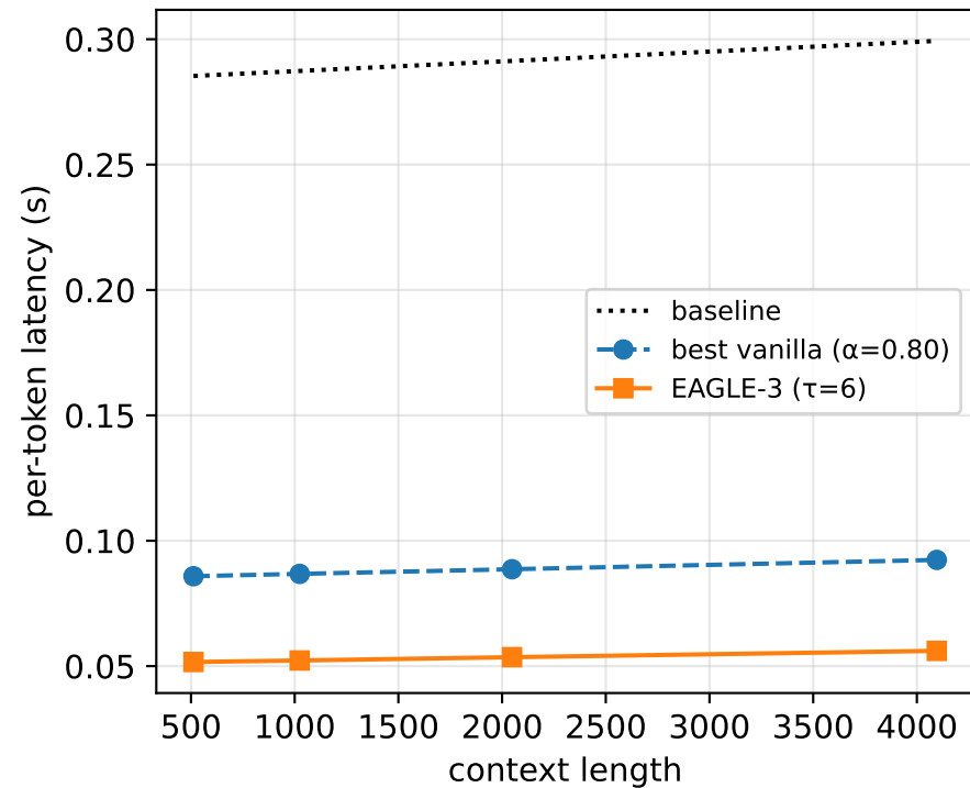
EAGLE-3 (calibrated \tau ) vs vanilla spec vs baseline (depth-aware)
