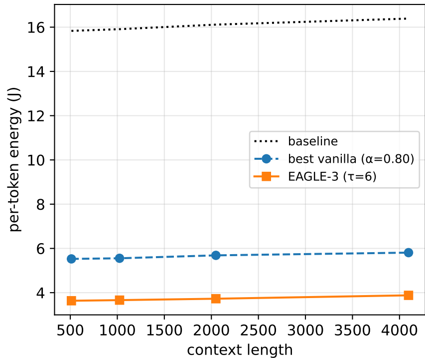
EAGLE-3 (calibrated \tau ) vs vanilla spec vs baseline (depth-aware)
