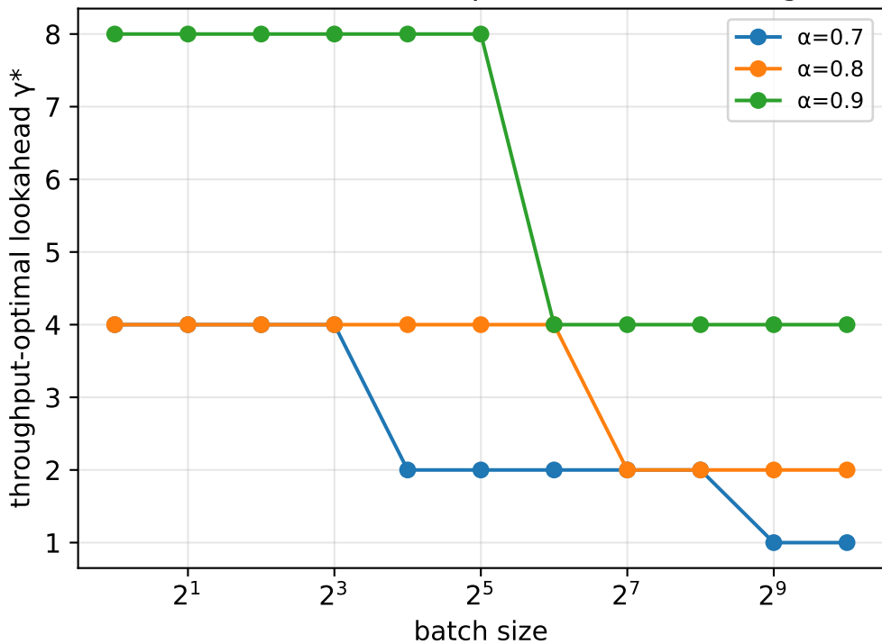
Load-aware lookahead: \gamma^* shrinks as batch grows
