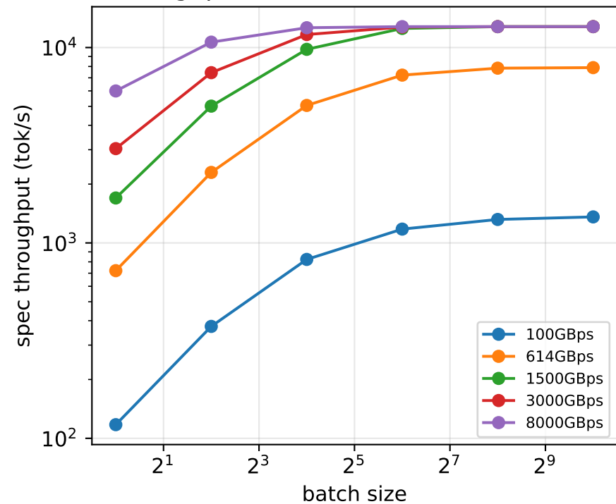
Throughput roofline vs DRAM bandwidth
