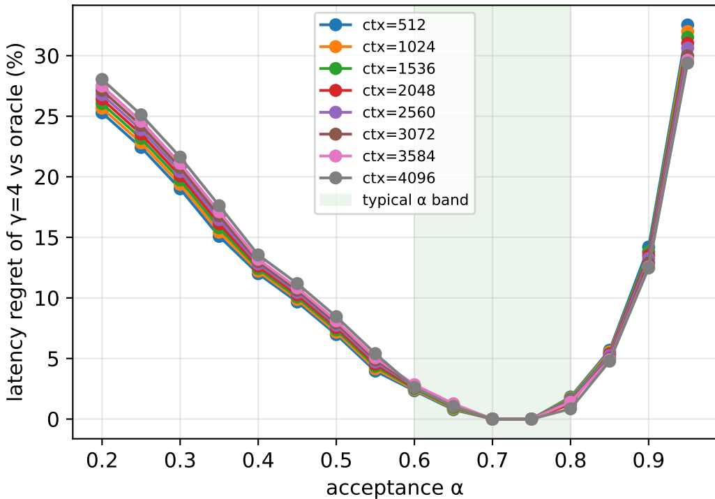
Static \gamma=4 is near-optimal in the typical \alpha band
