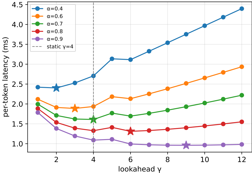
Latency vs \gamma is U-shaped; \gamma^* rises with \alpha (ctx=2048)
