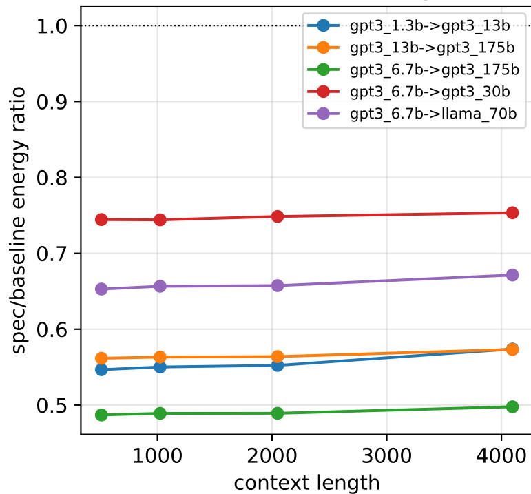
Speculative energy ratio ( \gamma=4 , \alpha=0.80 ) Model scale (draft→target)
