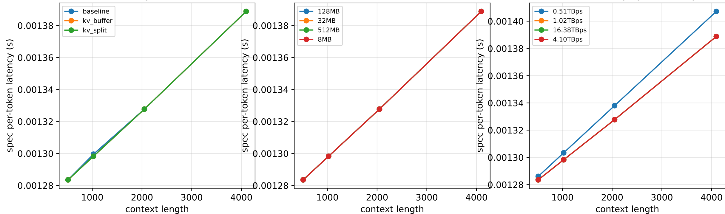
KV organization
