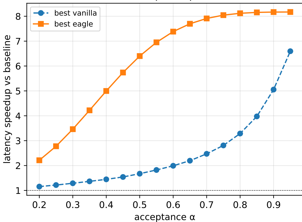
EAGLE-3 vs vanilla: speedup vs \alpha (ctx=2048)
