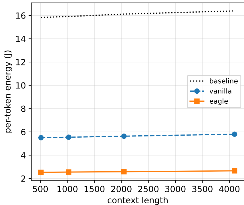
EAGLE-3 vs vanilla spec vs baseline (depth-aware, \alpha=0.80 )
