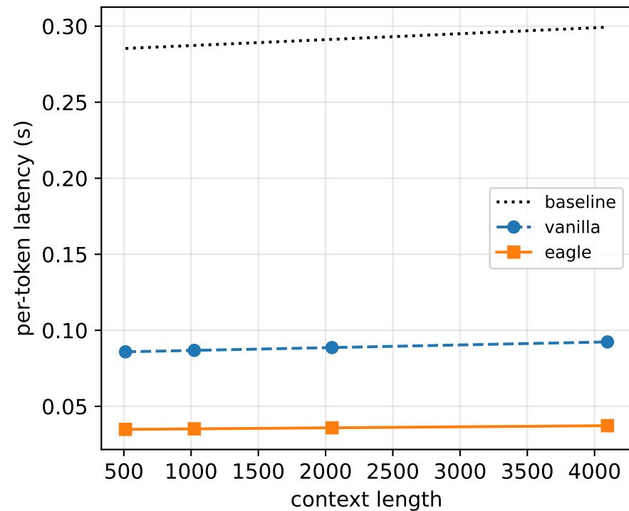
EAGLE-3 vs vanilla spec vs baseline (depth-aware, \alpha=0.80 )
