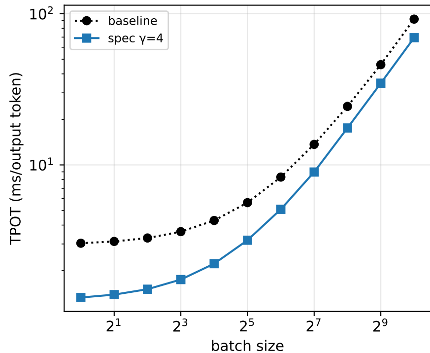
TPOT rises with batch ( \alpha=0.8 )
