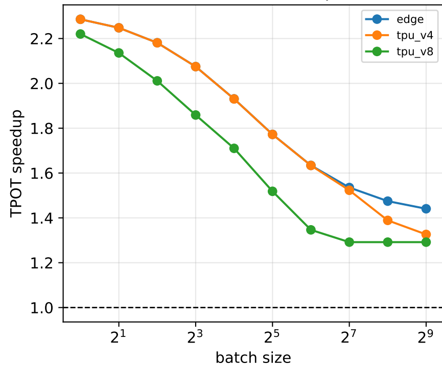
DRAM bandwidth shifts B^* ( \gamma=4 , \alpha=0.8 )
