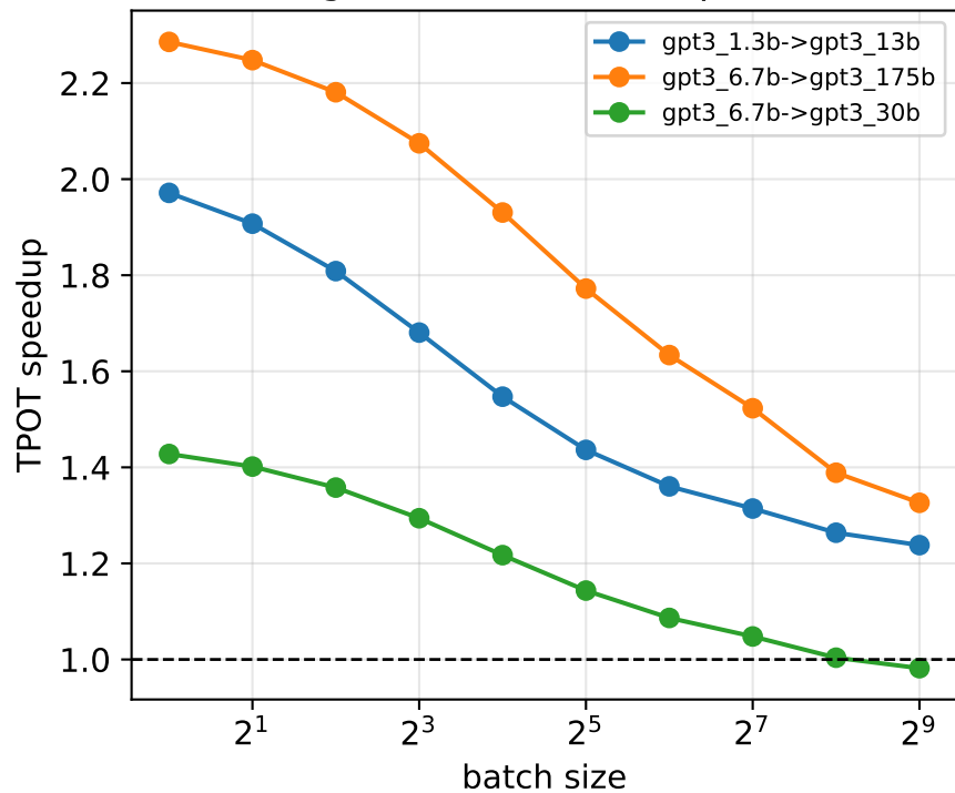
Draft/target ratio shifts B^* ( \gamma=4 , \alpha=0.8 )
