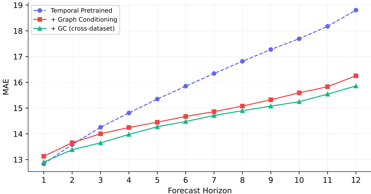
PEMS08 — MAE by Horizon
