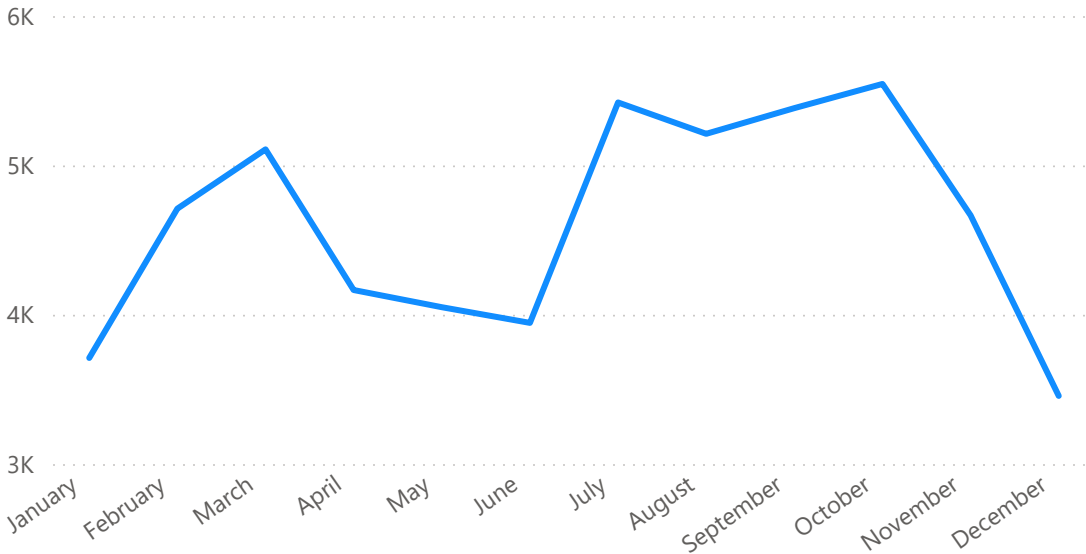
Number of Gap_Id by Month
