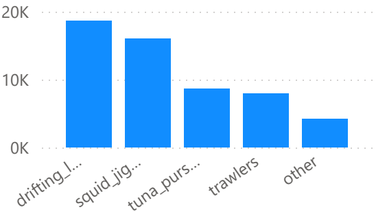
Number of Gap_Id vs Vessel Type
