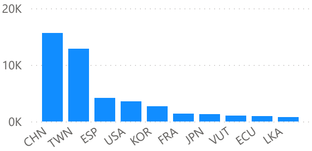
Number of Gap_Id by Flag
