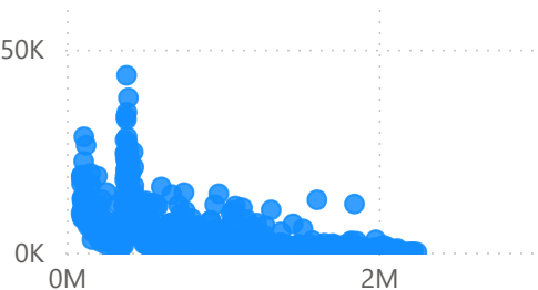
Sum of Gap Hour vs Gap Start Distance from Shore
