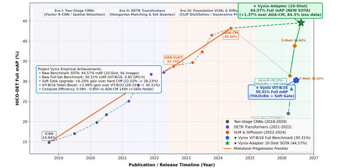
Fig. 1. Benchmark progression trajectory on HICO-DET (2018–2026) comparing fully supervised baselines against Project Vynix variants.
