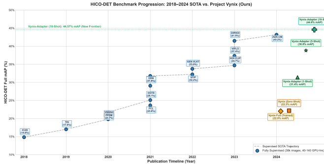
Fig. 1. Benchmark progression trajectory on HICO-DET (2018–2024) comparing fully supervised baselines against Project Vynix variants. Vynix-Adapter (10-Shot) establishes a new state-of-the-art of 44.57% mAP.
