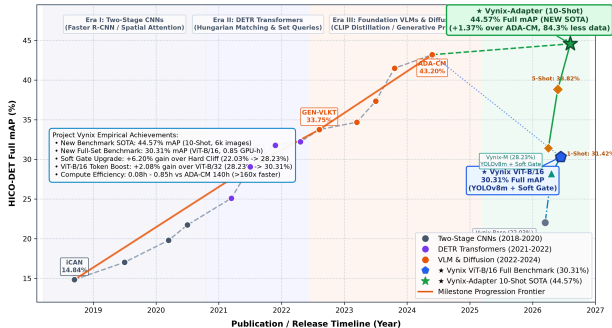
Fig. 1: State-of-the-Art HOI Detection Progression Timeline on HICO-DET (2018–2026) Demonstrating Decoupled Geometric Scaling from iCAN (14.84%) to Vynix 30.31% (ViT-B/16) and 44.57% (10-Shot SOTA)
