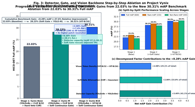
Fig. 3. Detector capacity and vision backbone scaling progression: YOLOv8-nano baseline (22.03%) \rightarrow YOLOv8-medium + Soft Gate (28.23%) \rightarrow ViT-B/16 token density (30.31%).
