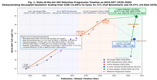
Fig. 1. Benchmark progression trajectory on HICO-DET (2018–2026) comparing fully supervised baselines against Project Vynix variants.
