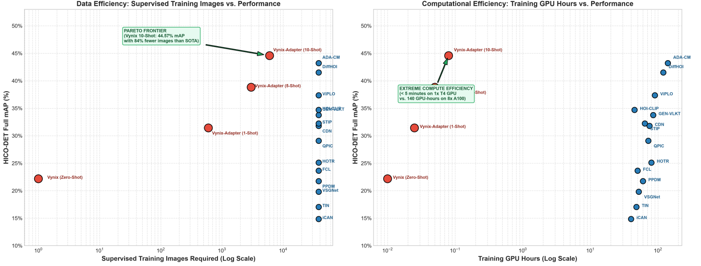
Fig. 3. Computational and Data Efficiency Pareto Frontiers. Left : Training images required vs. Full mAP. Right : Training GPU-hours vs. Full mAP. Vynix demonstrates extreme Pareto dominance in both axes.
