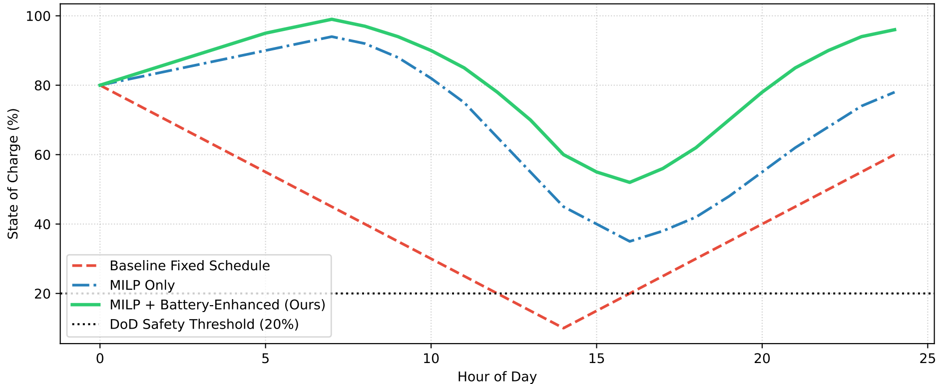
24-Hour Battery SoC Trajectory Comparison
