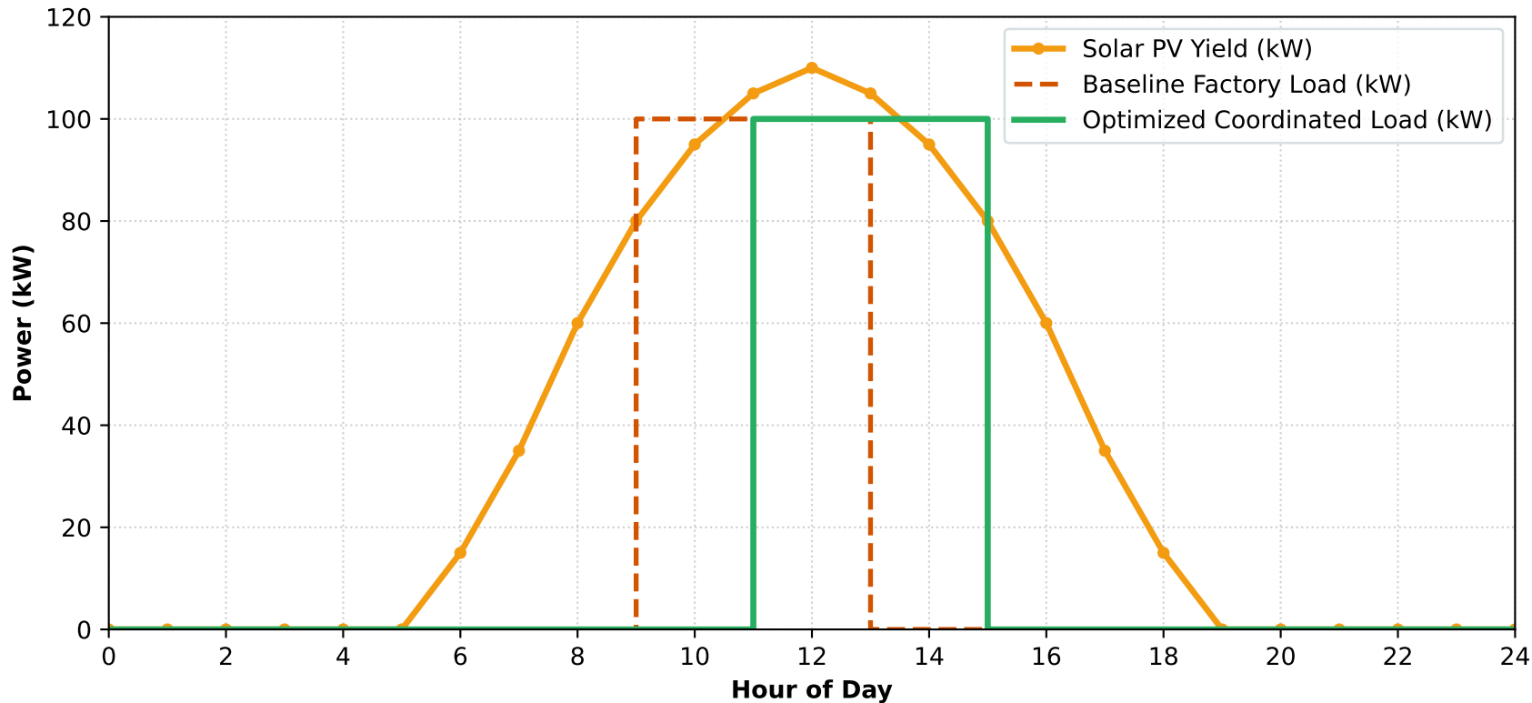
24-Hour Solar Yield and Active Load Scheduling Comparison
