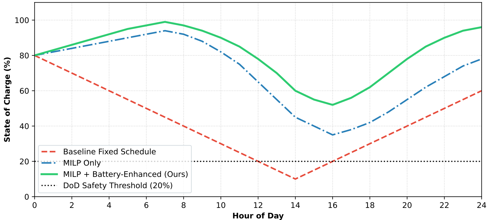
24-Hour Battery SoC Trajectory Comparison
