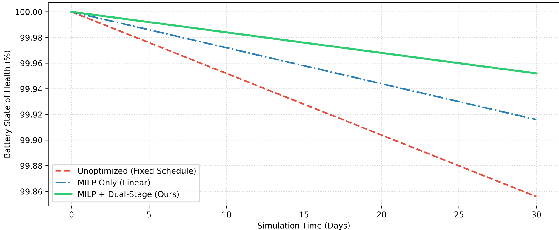
30-Day Battery SoH Capacity Fade Comparison
