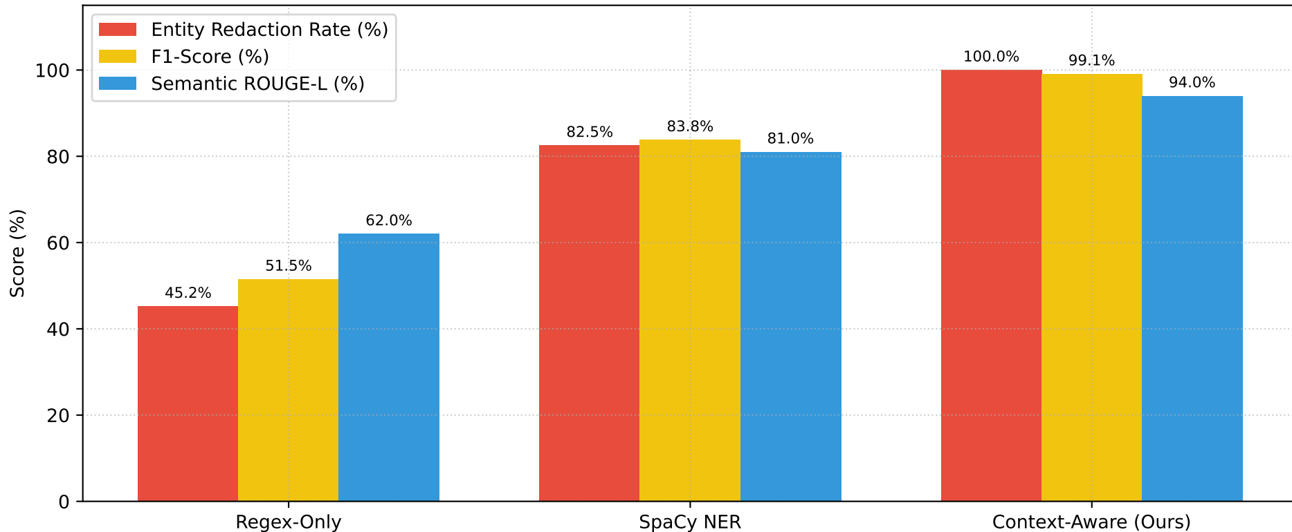
Privacy Shield Anonymization & Utility Metrics Comparison
