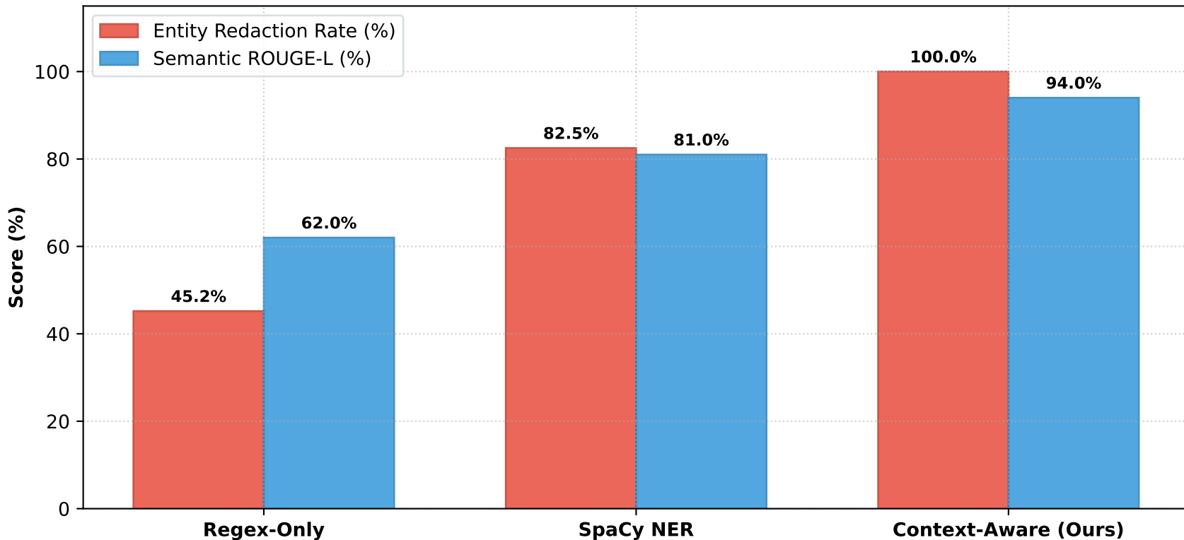
Privacy Shield Anonymization & Utility Metrics Comparison
