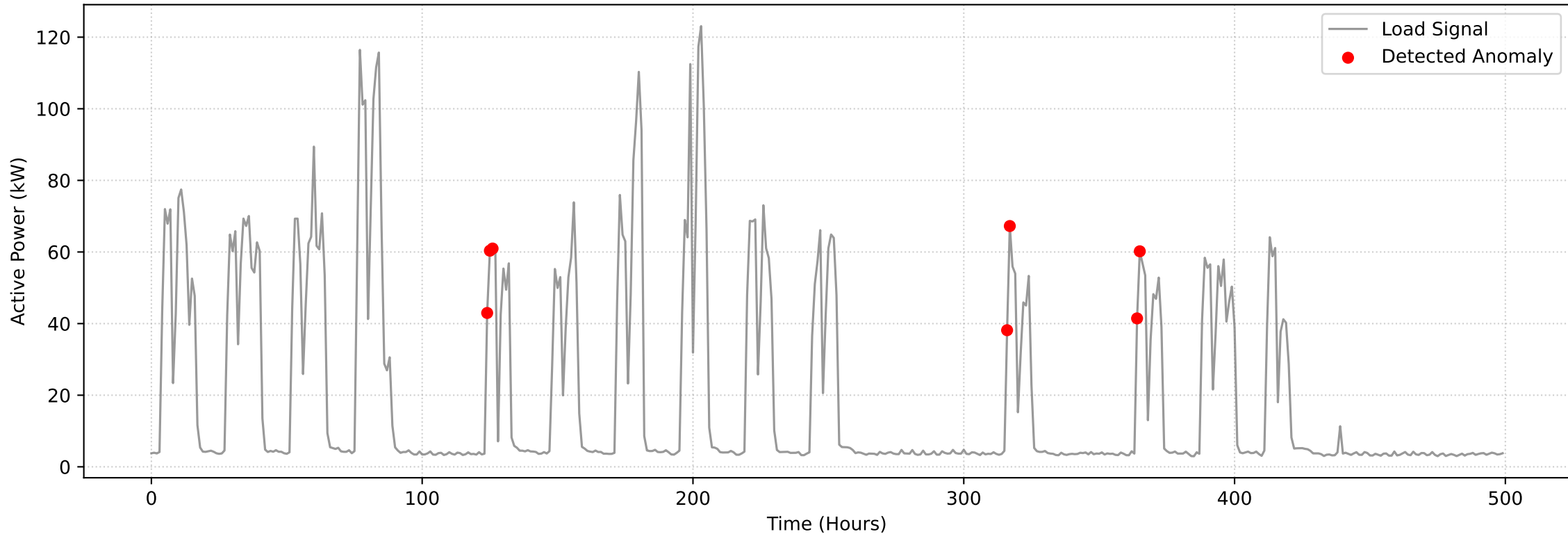
TC-iForest Anomaly Detection on UCI Steel Dataset
