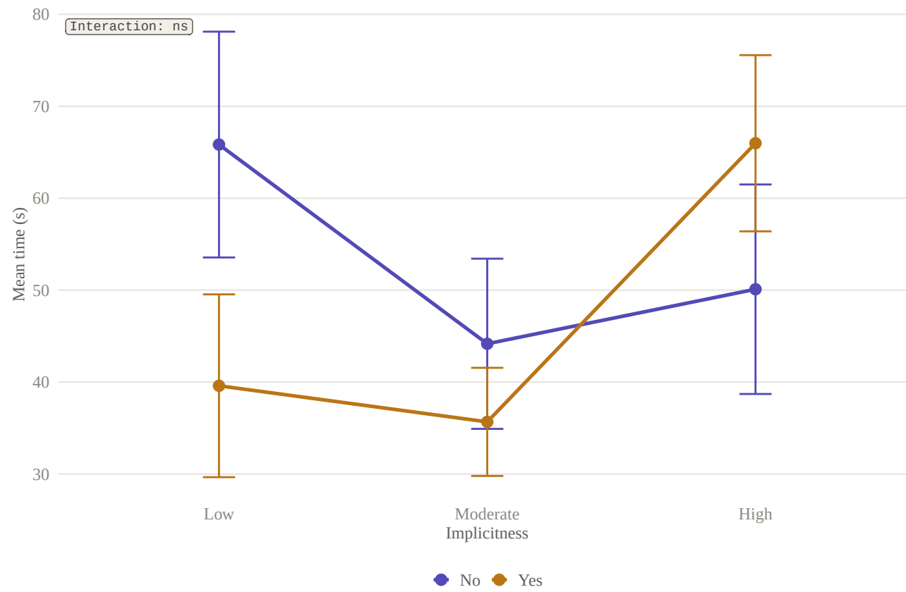
L6 Time Interaction
