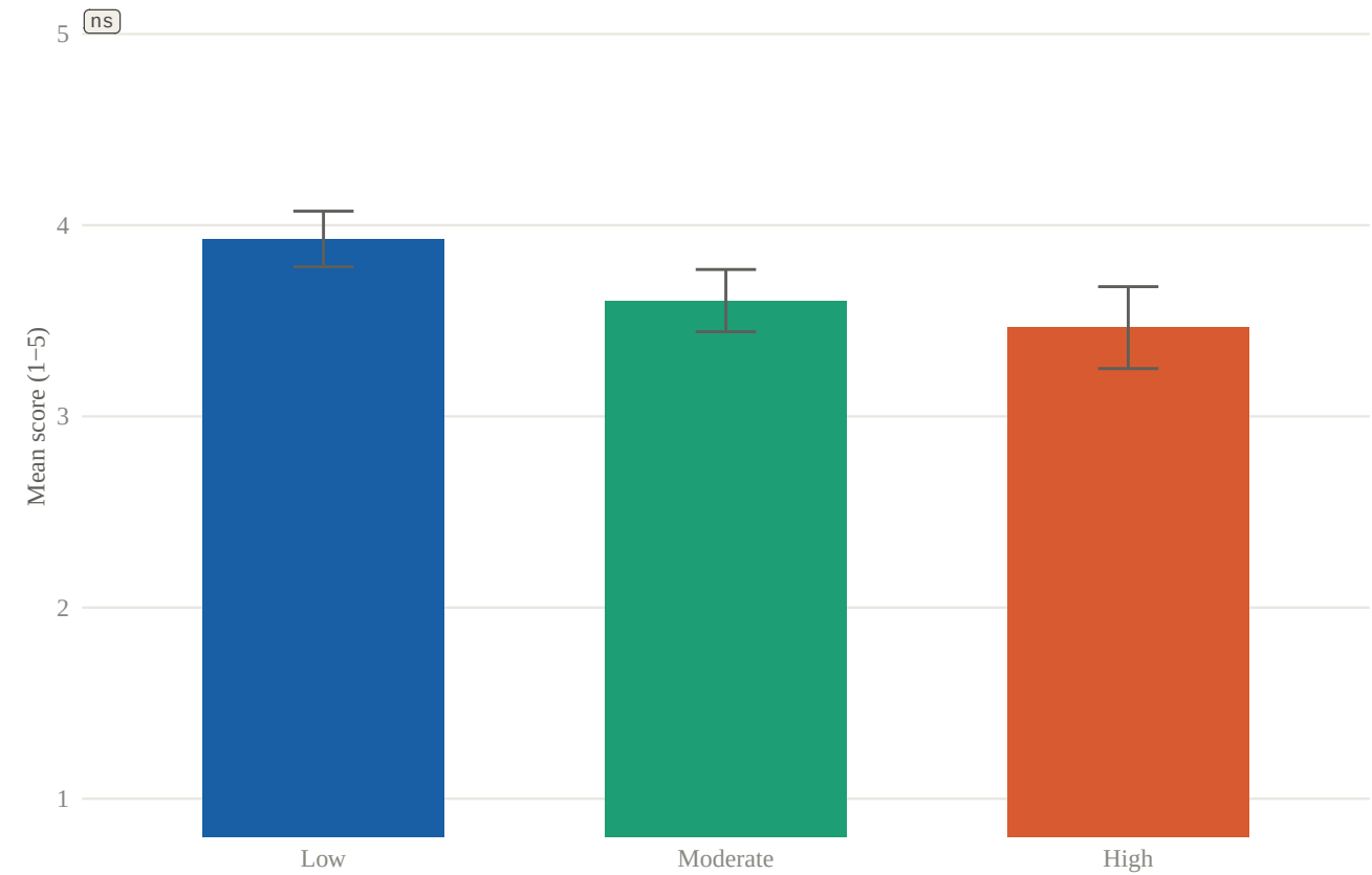
Clarity by Implicitness
