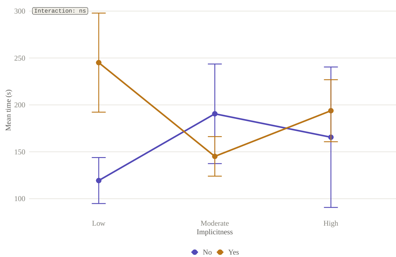
L7 Time Interaction
