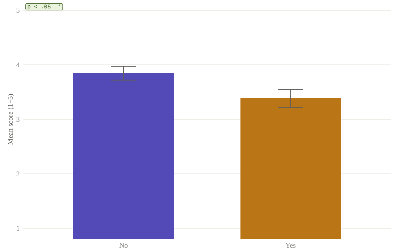
Clarity by Adaptability
