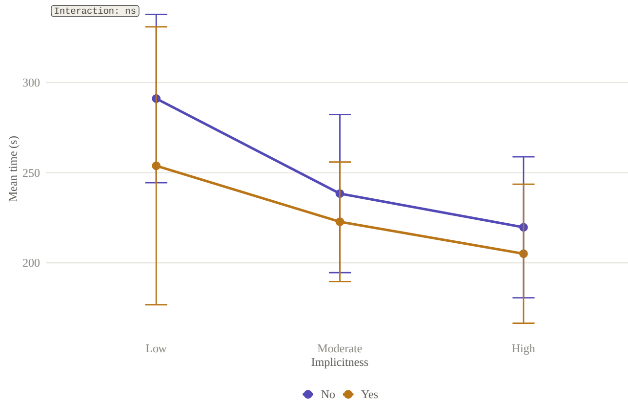
Total Time Interaction
