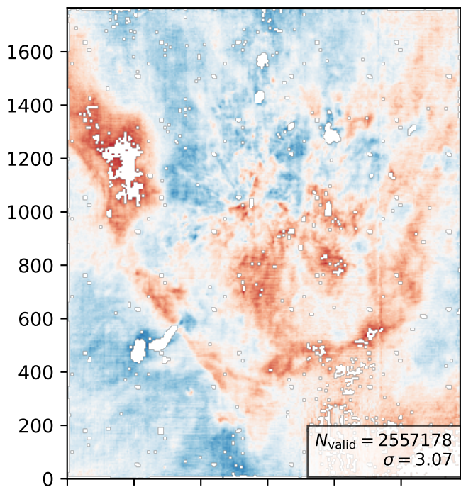
[\text{ArIII}] \lambda 7136
