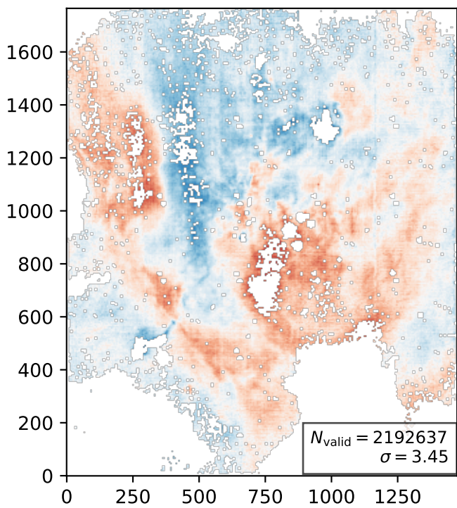
[\text{ArIII}] \lambda 7136
