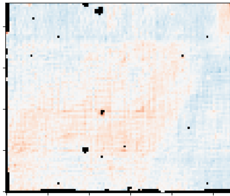
H \alpha bin 16
