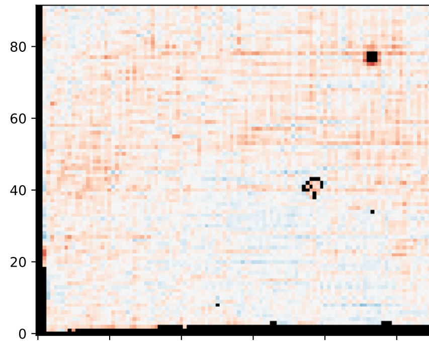
H \alpha bin 8
