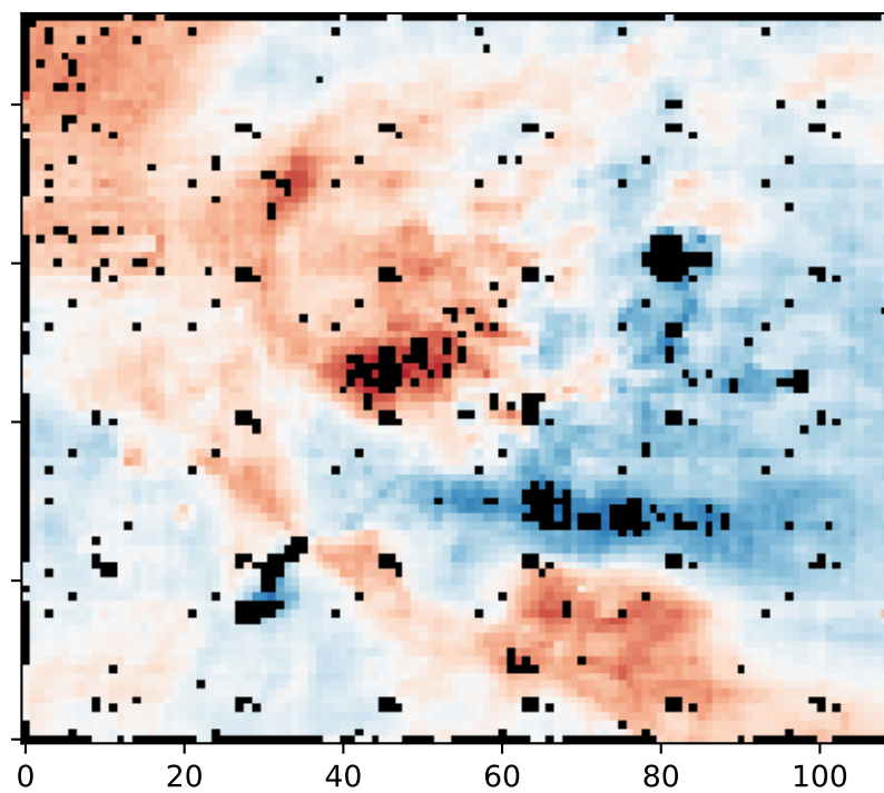
H \alpha bin 16
