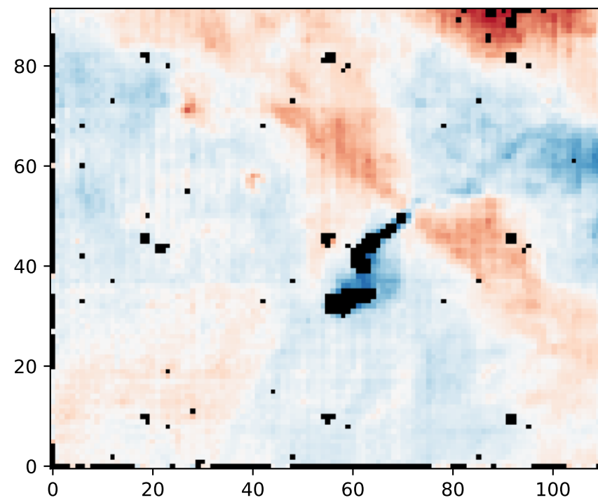
H \alpha bin 8
