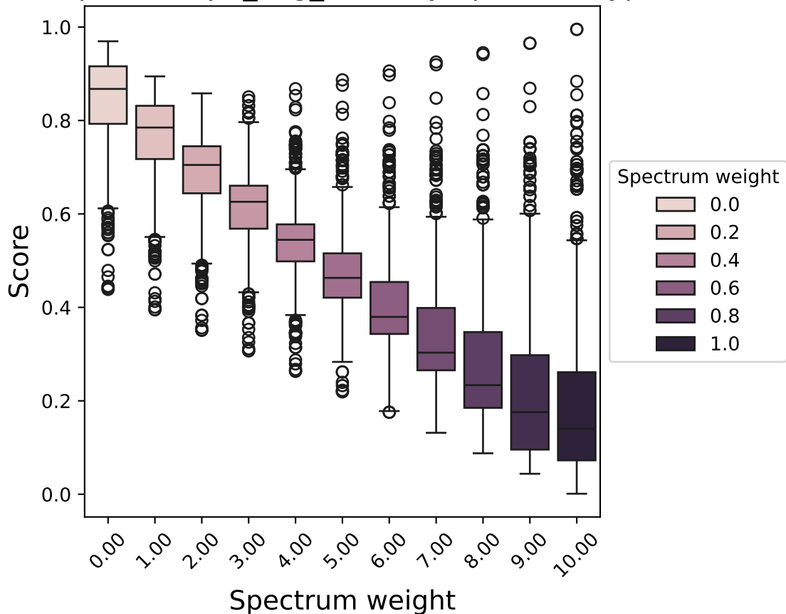
Boxplot of top2_avg_score by Spec Sim Type
