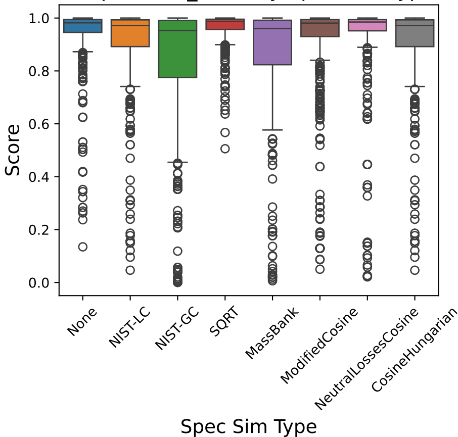
Boxplot of H_{\text{norm}} by Spec Sim Type
