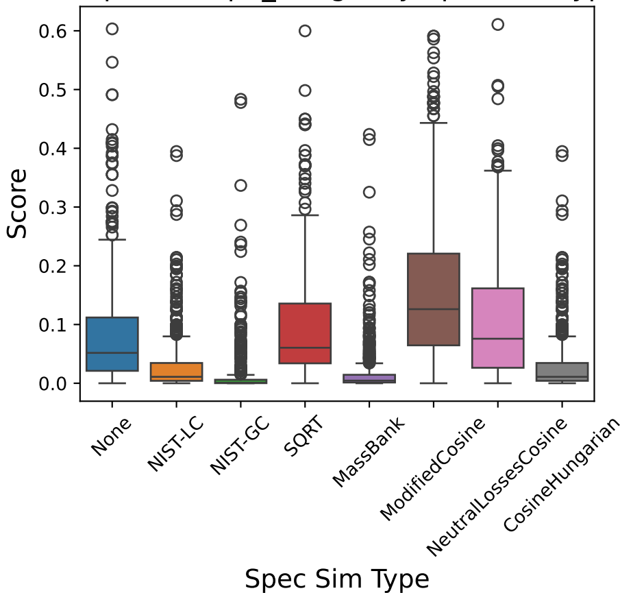
Boxplot of top1_margin by Spec Sim Type
