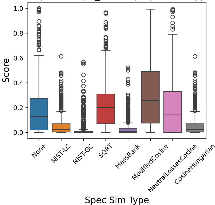
Boxplot of top1_score by Spec Sim Type
