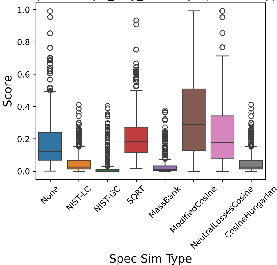
Boxplot of top3_avg_score by Spec Sim Type
