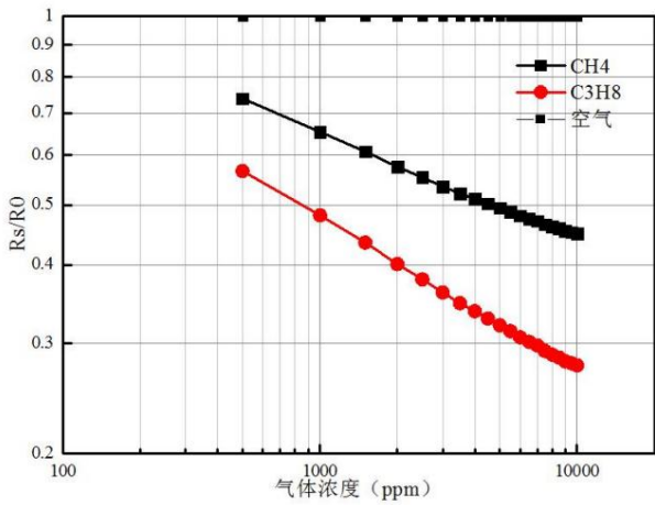
Figure 3. Typical logarithmic sensitivity characteristic curve of the sensor.
