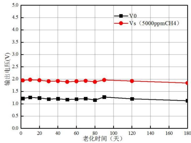
Figure 7 Long-term stable characteristic curves
