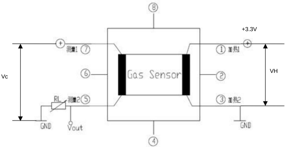
Figure 2 GM-402B test circuit
