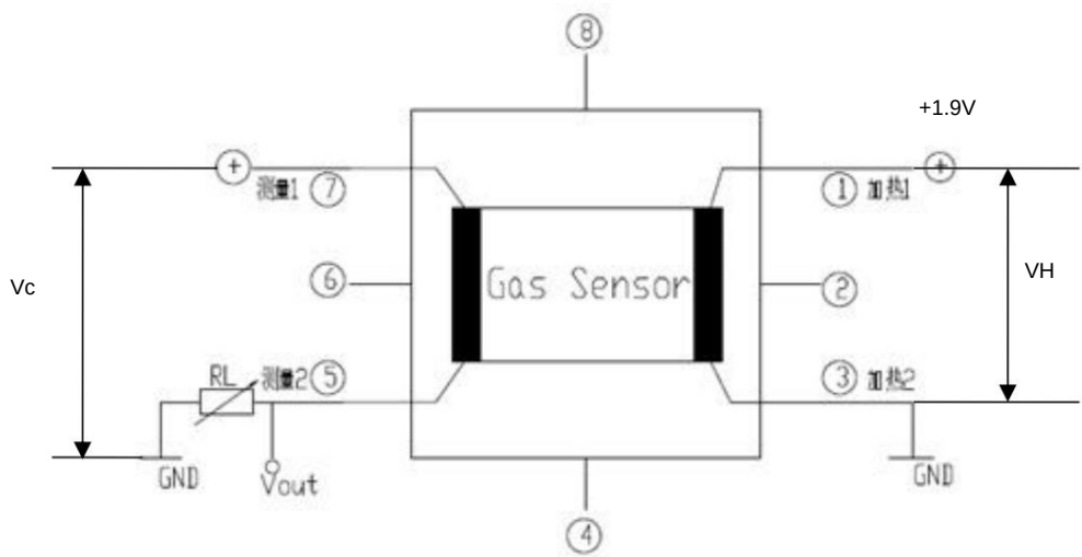
Figure 2 GM-602B Test Circuit
