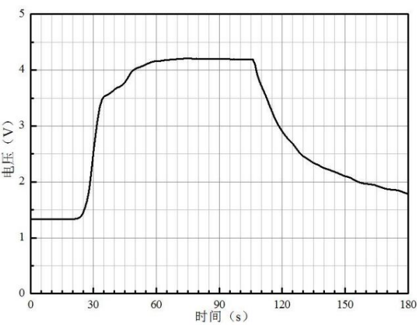
Figure 5 Response recovery curve
