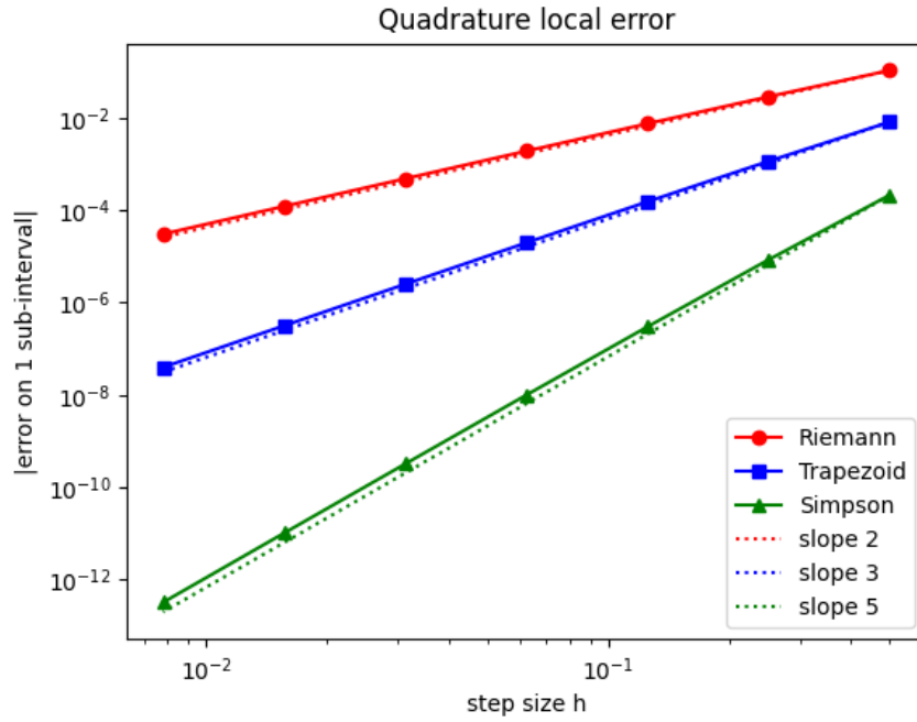
Figure 9: Local (one sub interval) error of each quadrature rule vs step size h . Dotted lines show slopes 2, 3, 5 for comparison. Fitted slopes: Riemann 1.97, trapezoid 2.95, Simpson 4.90, matching the local truncation error from Section 4.
