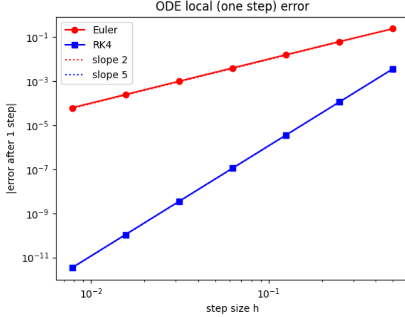
Figure 5: Local (one step) error of Euler and RK4 vs step size h . Dotted lines show slopes 2 and 5 for comparison. Fitted slopes: Euler 1.99, RK4 4.99, matching the local truncation error from Section 4.
