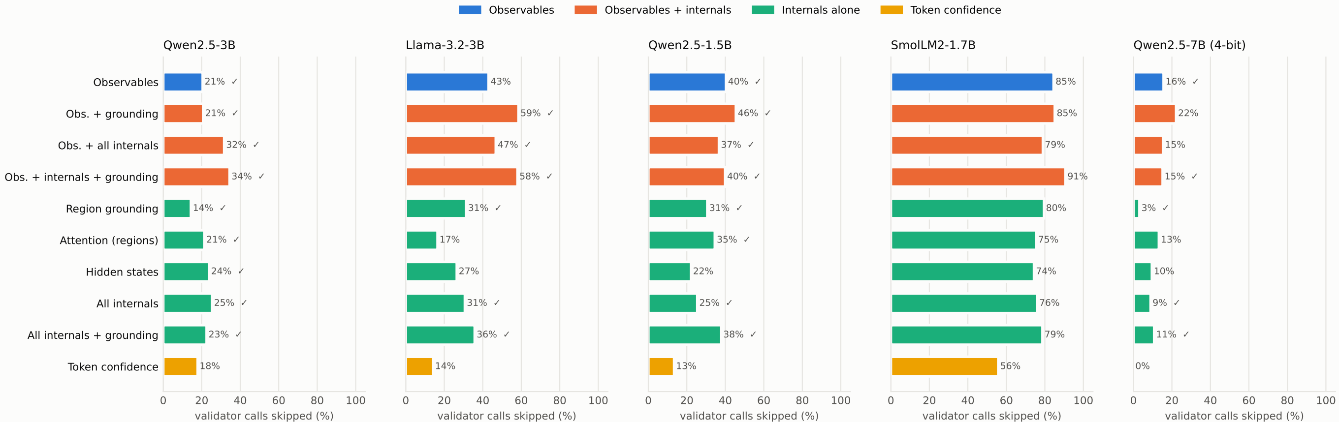
FSM: validator calls skipped per signal (fresh certification set, X = 10%)
