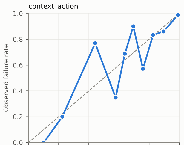
Reliability (dev_thr) (dashed: perfect calibration; bins with n < 5 hidden)
