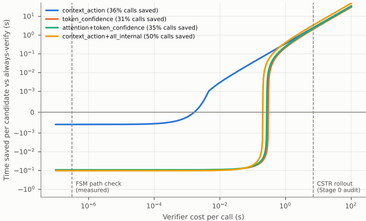
Time saved vs verifier cost (point, \alpha = \beta = 0.1 ; FSM routing and overhead)
