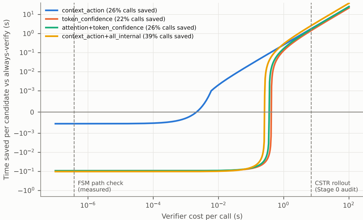
Time saved vs verifier cost (point, \alpha = 0.01 , \beta = 0.1 ; FSM routing and overhead)
