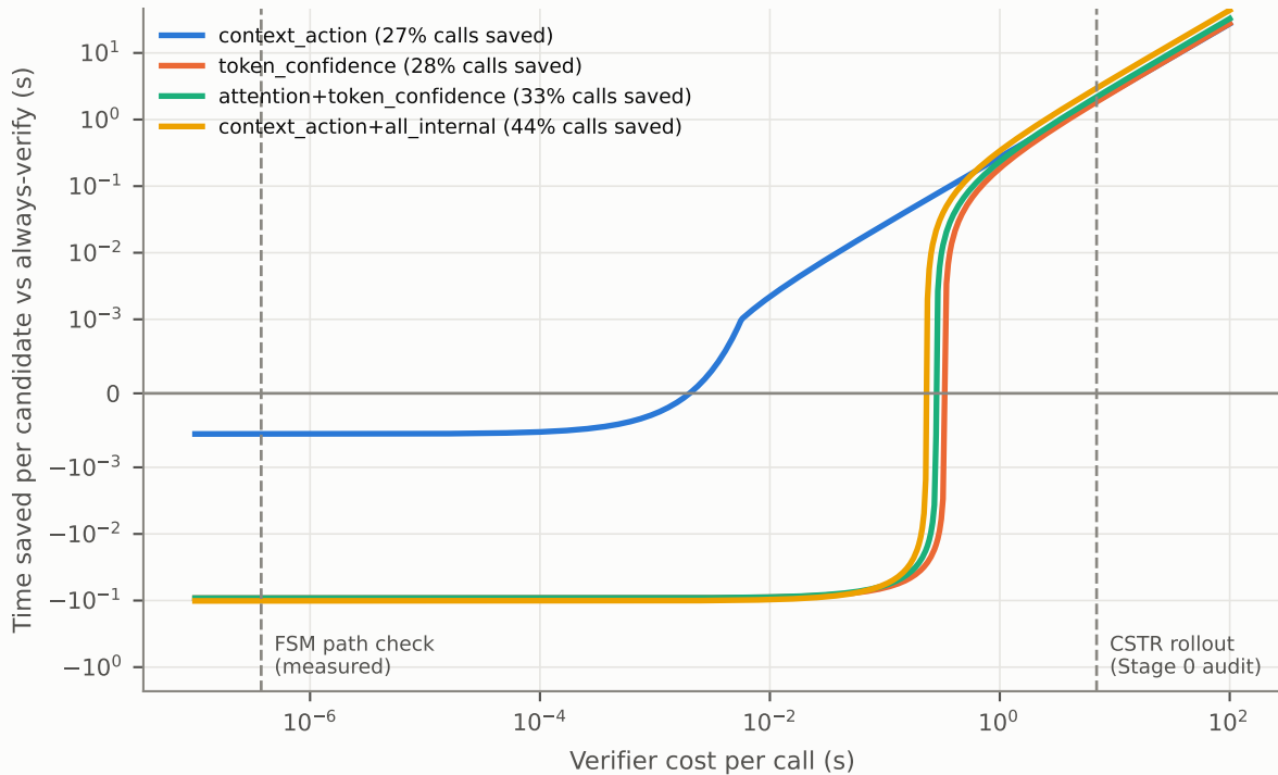
Time saved vs verifier cost (point, \alpha = 0.05 , \beta = 0.1 ; FSM routing and overhead)
