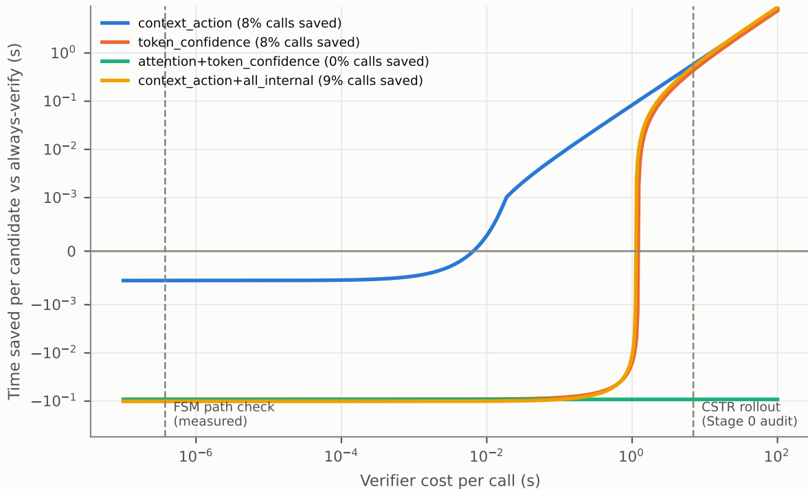
Time saved vs verifier cost (ucb, \alpha = 0.01 , \beta = 0.1 ; FSM routing and overhead)
