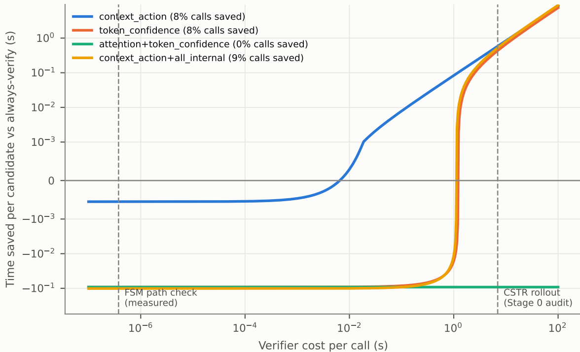
Time saved vs verifier cost (ucb, \alpha = 0.02 , \beta = 0.1 ; FSM routing and overhead)
