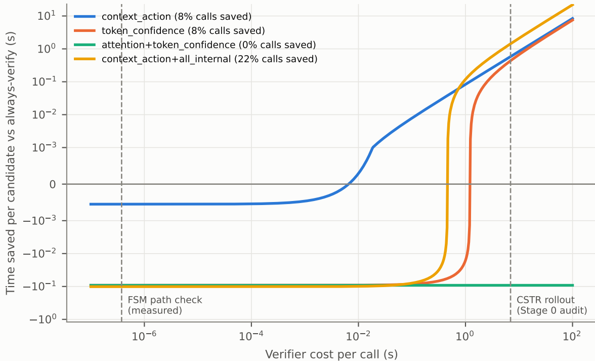
Time saved vs verifier cost (ucb, \alpha = 0.05 , \beta = 0.1 ; FSM routing and overhead)
