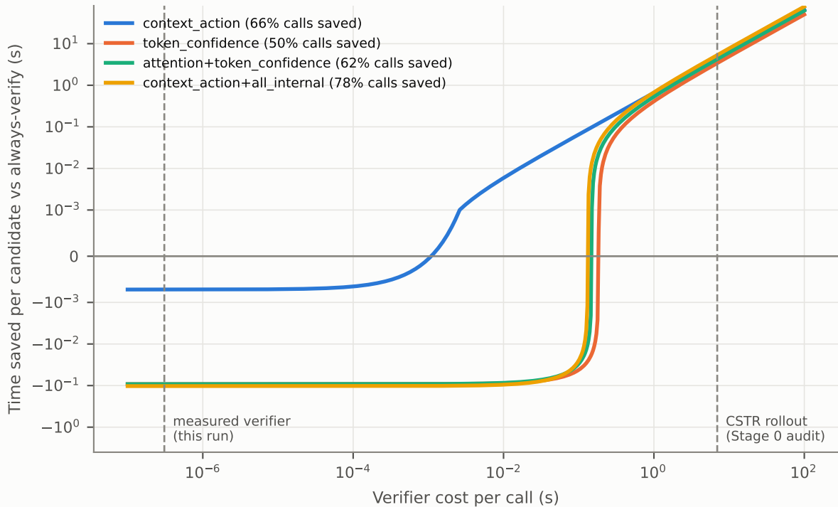
Time saved vs verifier cost (point, \alpha = 0.2 , \beta = 0.2 ; FSM routing and overhead)
