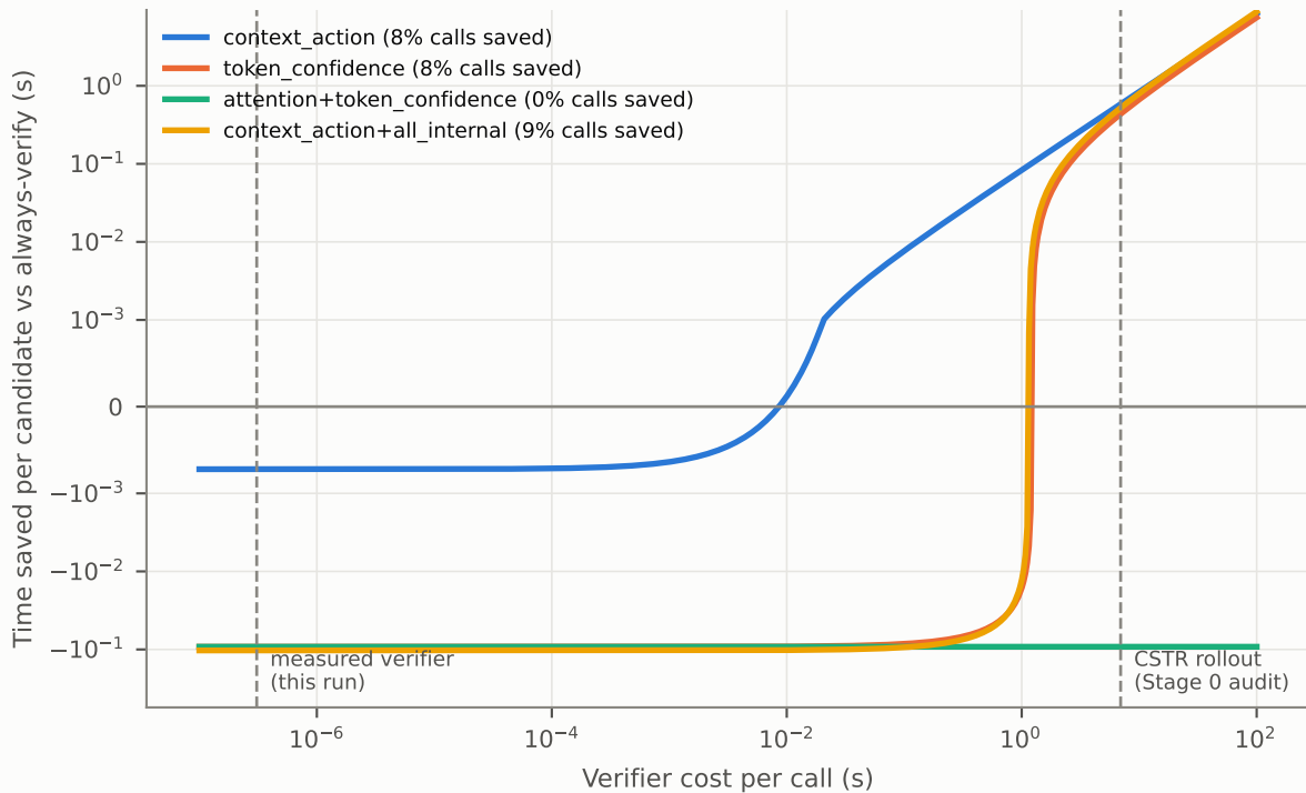
Time saved vs verifier cost (ucb, \alpha = 0.0 , \beta = 0.1 ; FSM routing and overhead)
