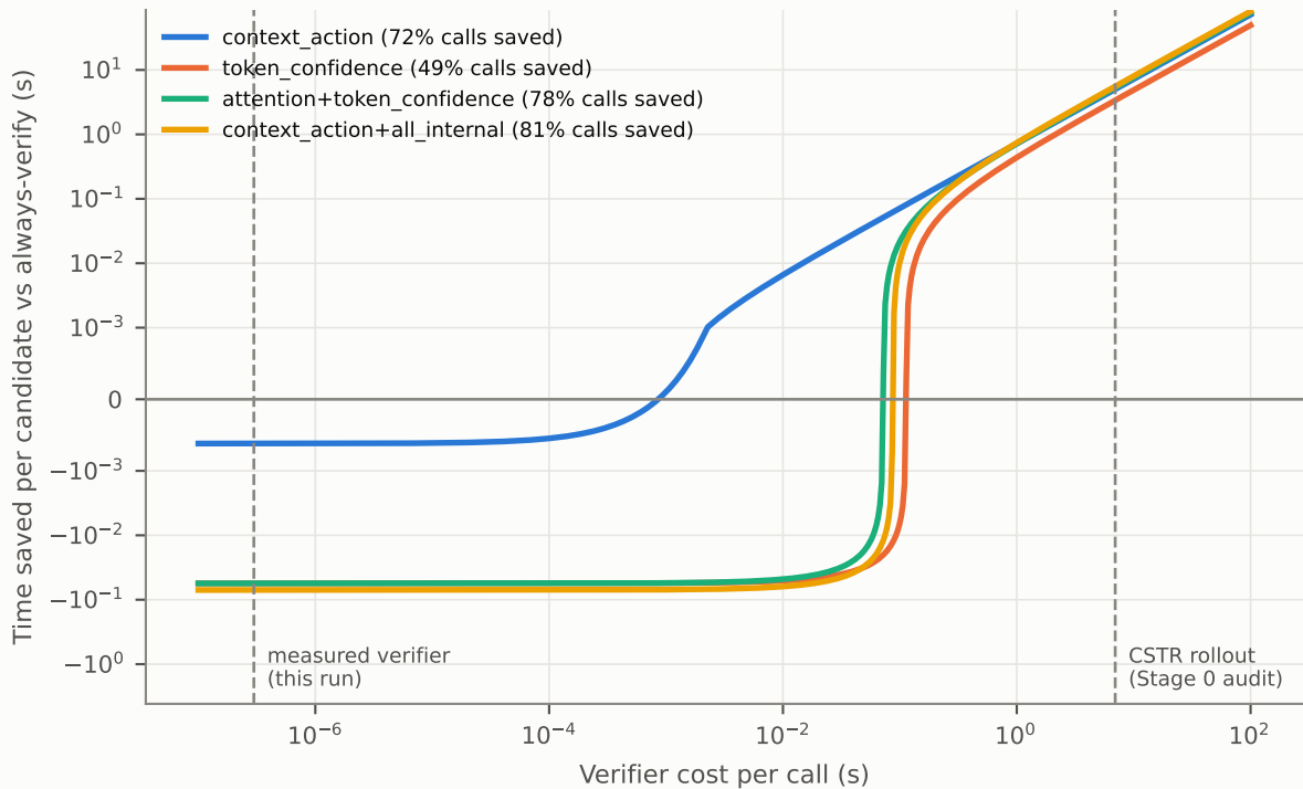
Time saved vs verifier cost (ucb, \alpha = 0.2 , \beta = 0.2 ; FSM routing and overhead)
